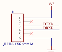
DPI interface - console port
